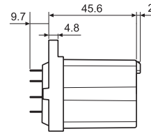
062.10 with relay
